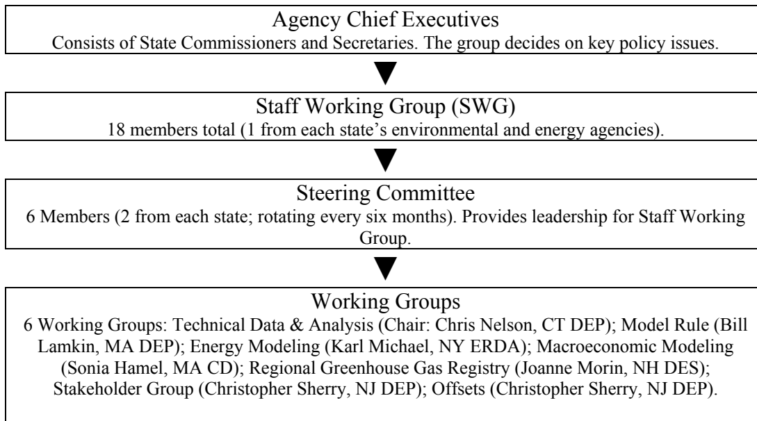
Figure 1: RGGI Structure
